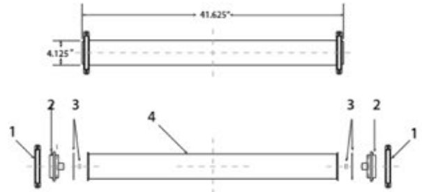
SPV-4040-12 Front View
